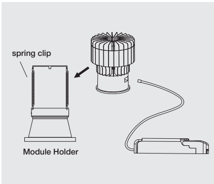
4. Attach module to module holder with spring clip and connect module to driver.
