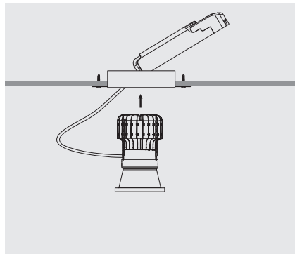
5. Gently insert module holder from the bottom of the trimless kit.
