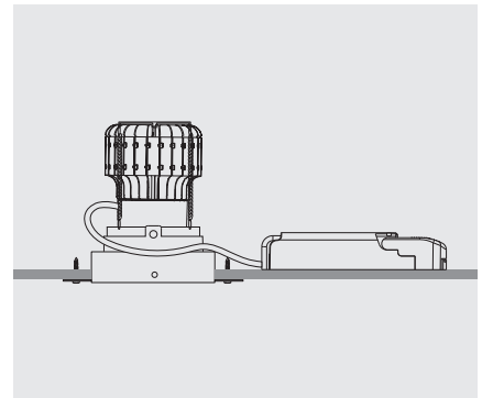
6. Installation complete.
